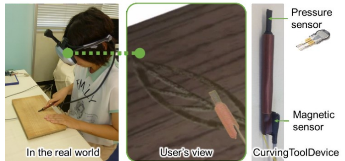
Figure 1: MR carving system
