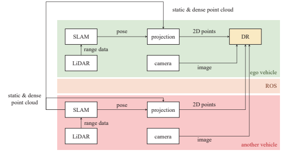
Figure 2: Dataflow of the current experiment.
