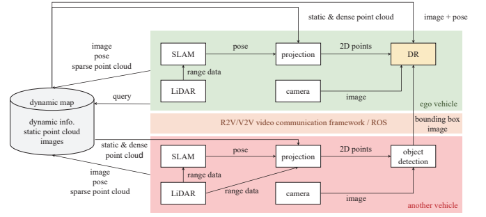
Figure 1: Dataflow of the future system.
